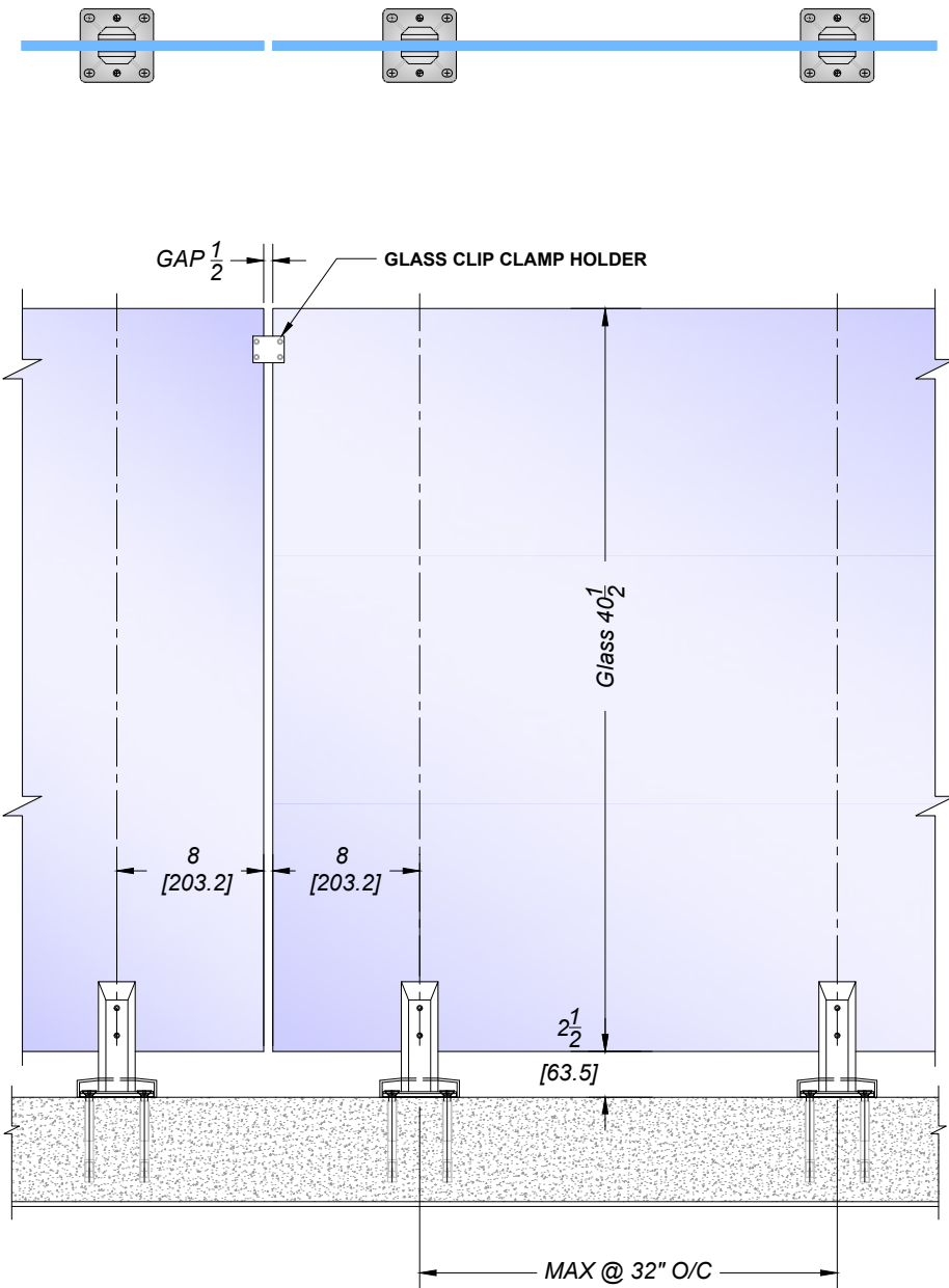
ELEVATION FOR GLASS RAILING SYSTEMS
