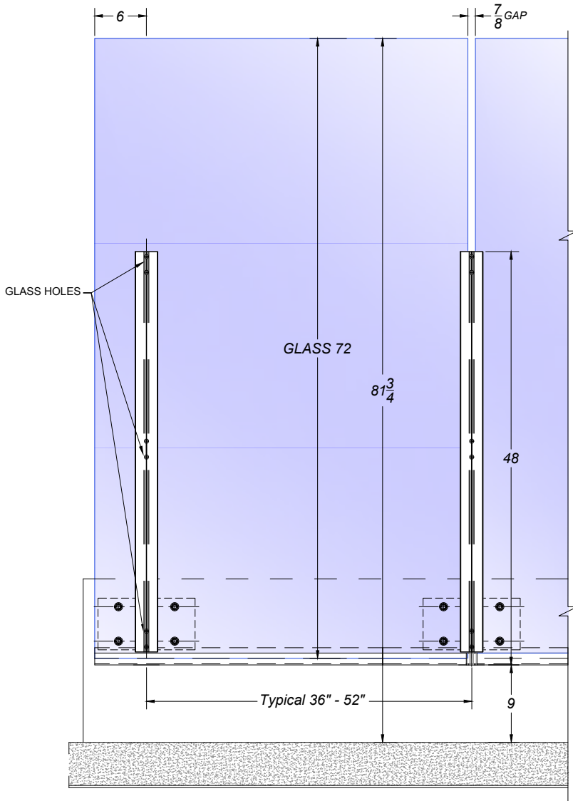
ELEVATION FOR GLASS WINDSCREEN SYSTEMS
