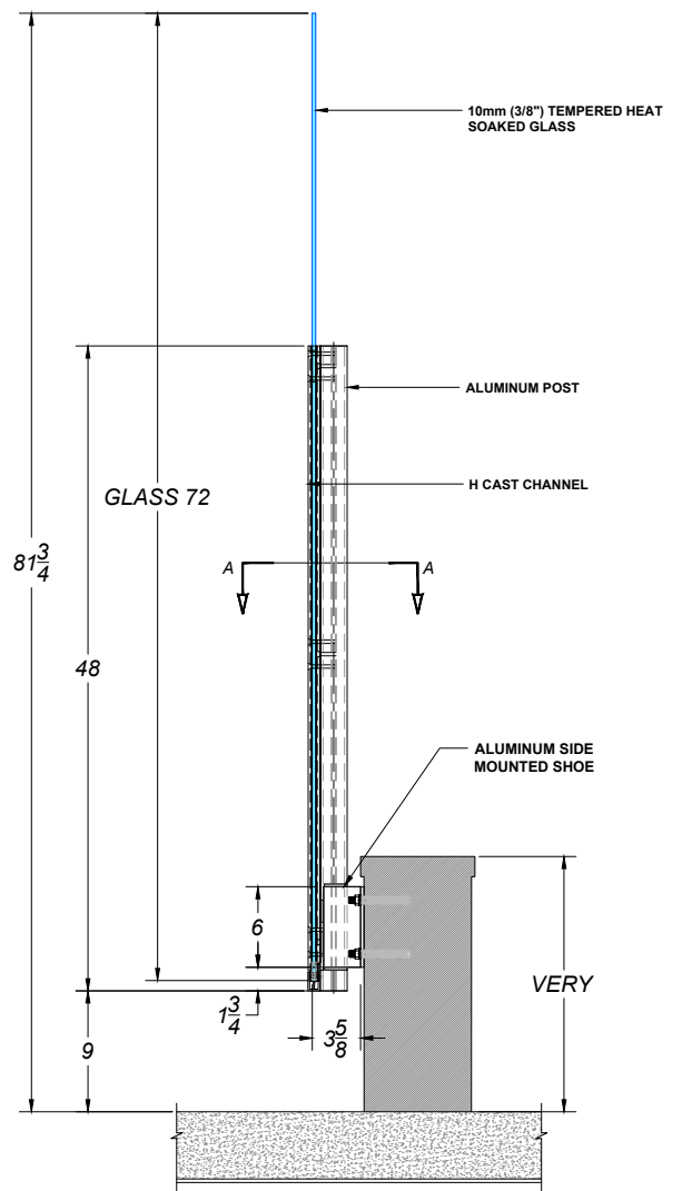
GLASS WINDSCREEN SECTION
