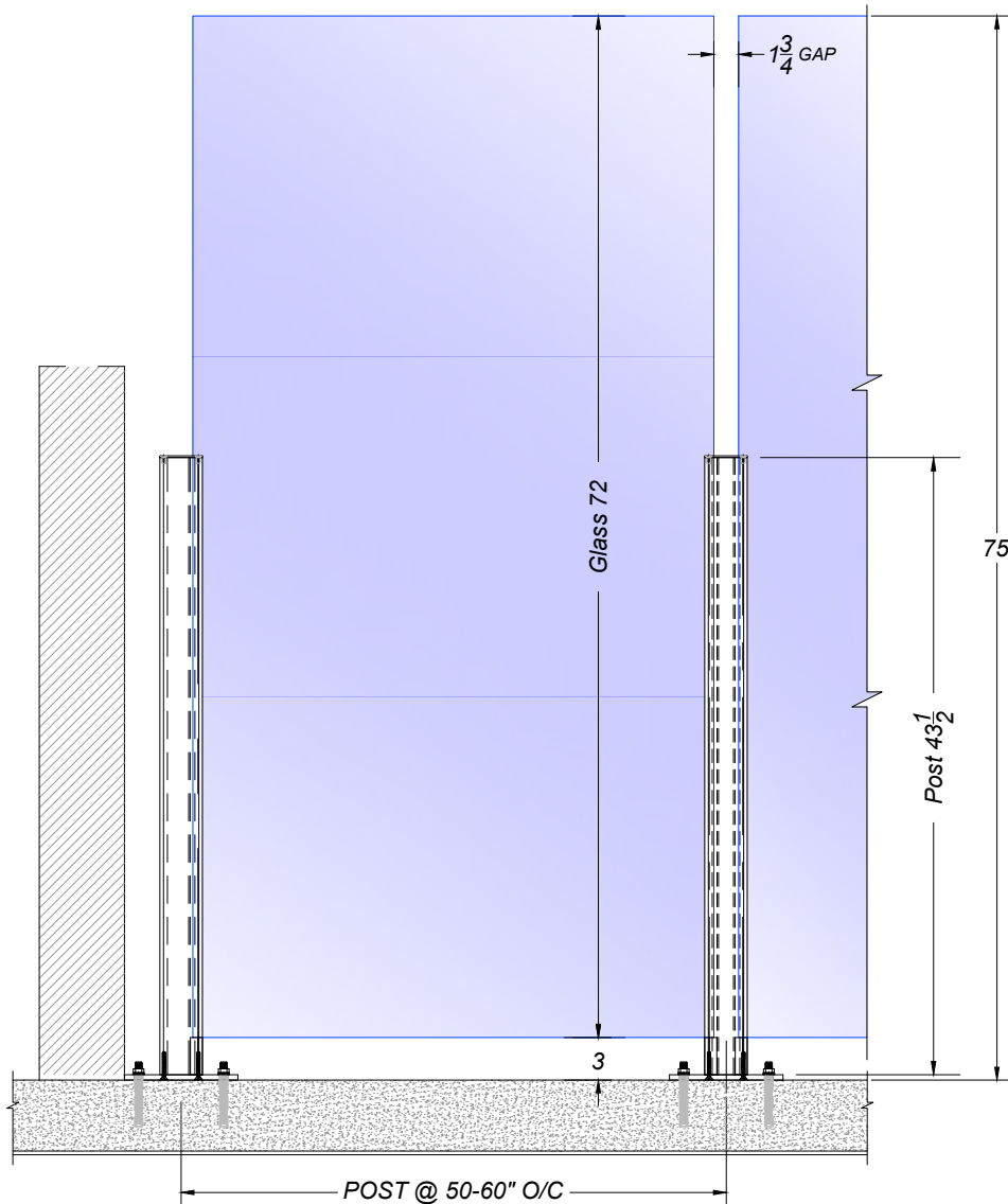
ELEVATION FOR GLASS WINDSCREEN SYSTEMS
