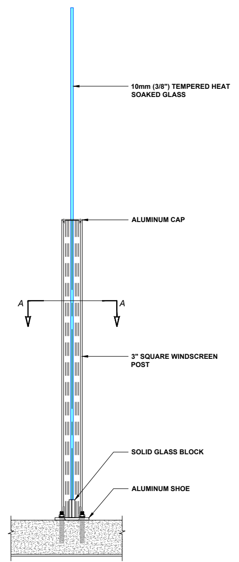
GLASS WINDSCREEN SECTION
