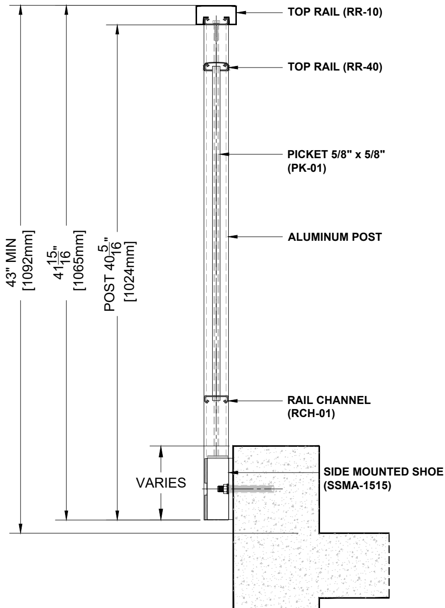
SIDE-MOUNTED/ PICKET RAILING RR-10 ASSEMBLY SECTION VIEW
