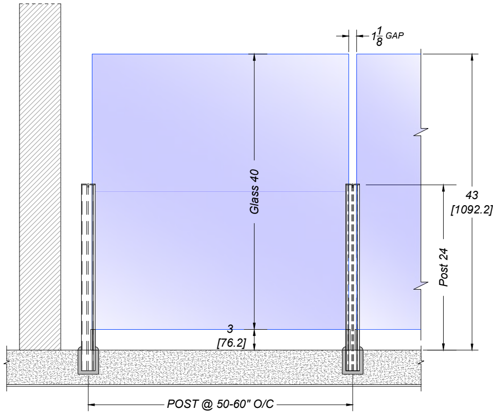
ELEVATION FOR GLASS RAILING SYSTEMS
