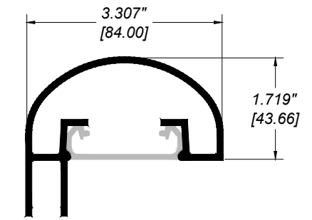
RR-60A TOP RAIL
