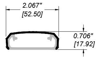
RR-40 TOP RAIL
