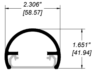
RR-70 TOP RAIL
