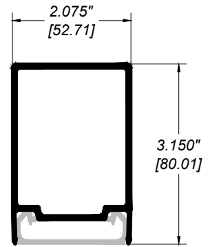
RR-30 TOP RAIL
