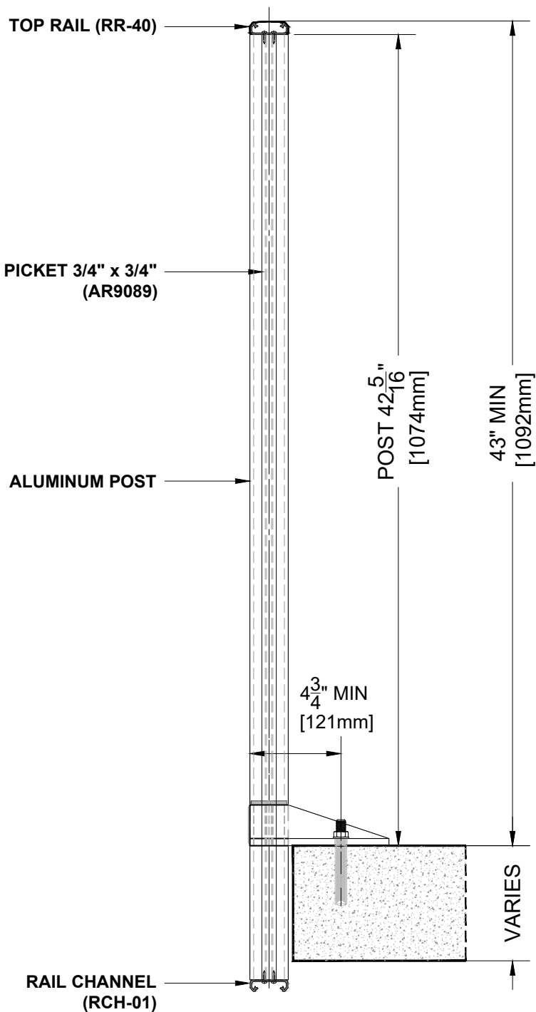
BALCONY RAILING SECTION
