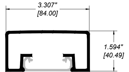
RR-10 TOP RAIL
