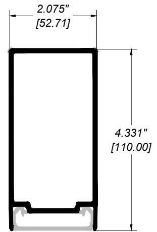
RR-20 TOP RAIL
